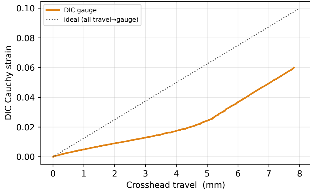
Gauge strain vs crosshead
